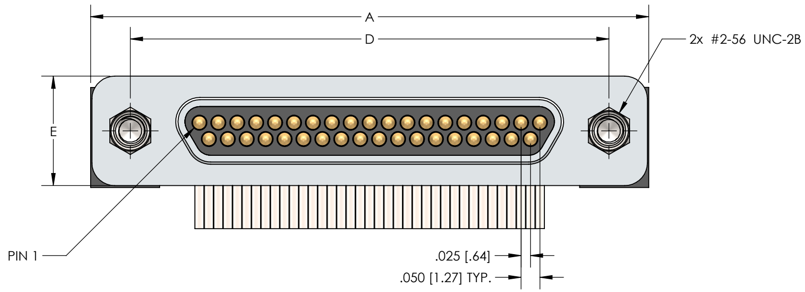
FRONT VIEW - PLUG (PINS)
